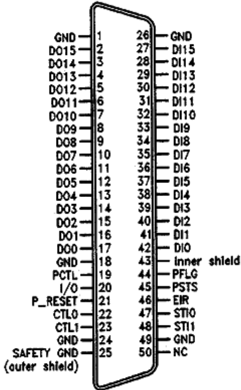
TAMS 61622 GPIO Connector Pinouts
